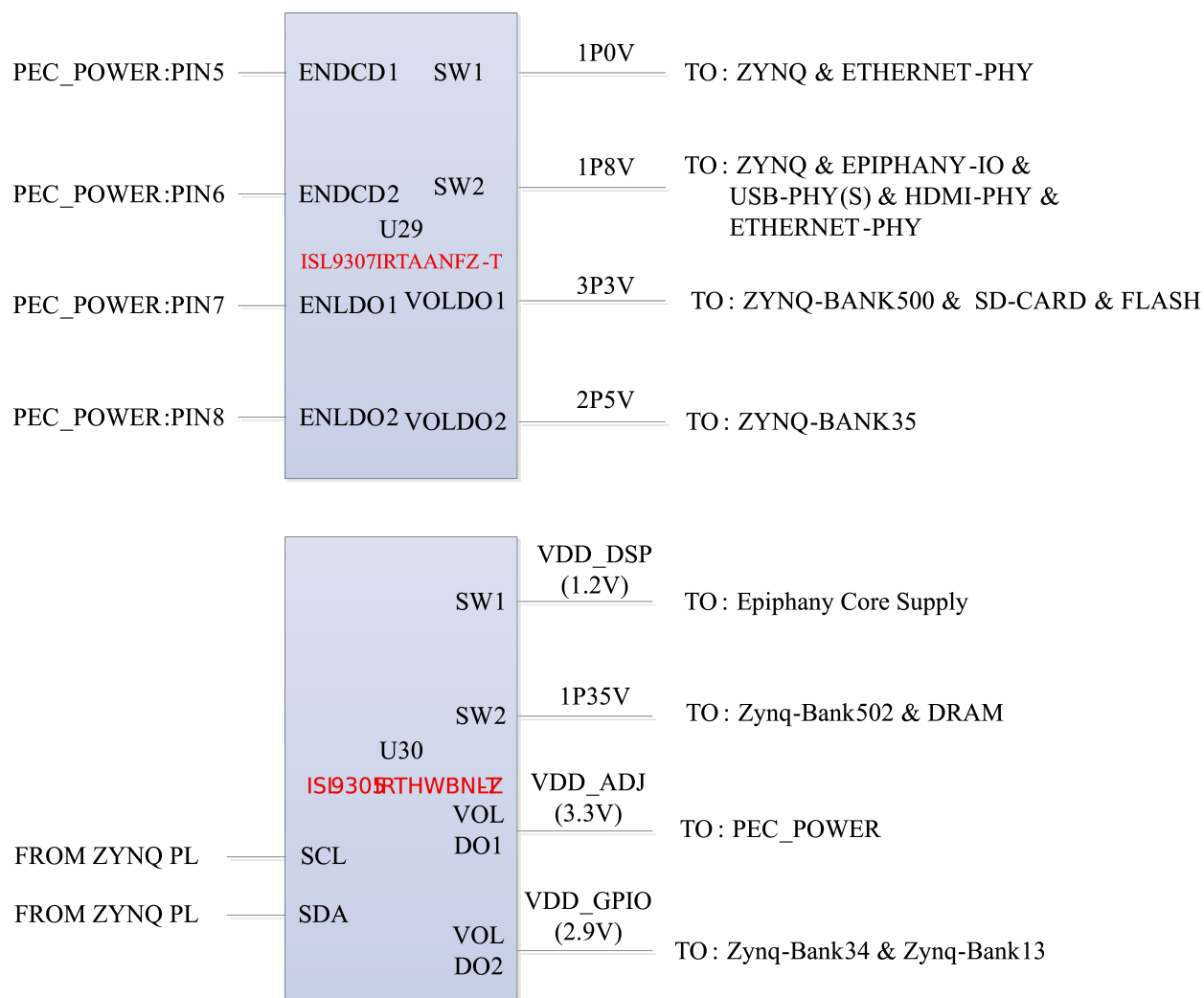
Figure 4: Power Sub-System
