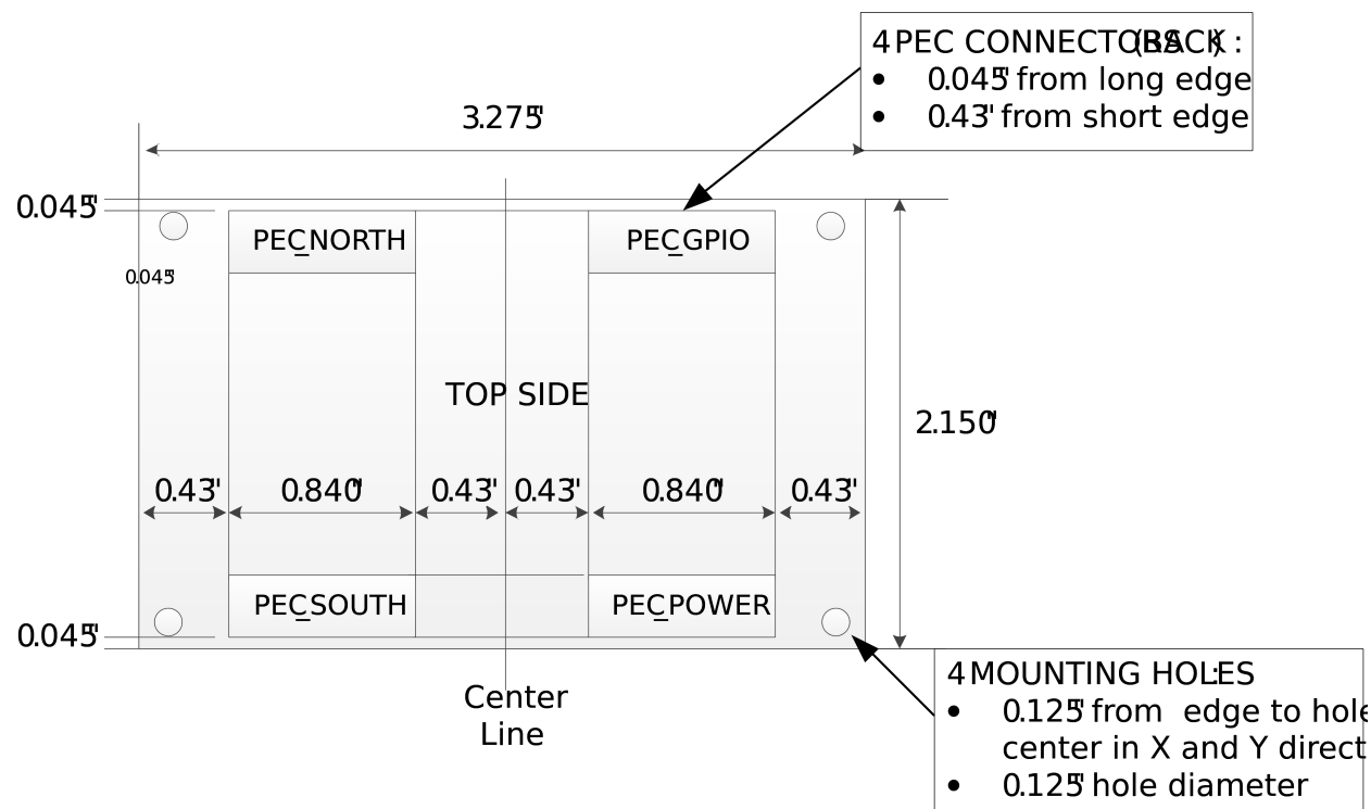
Figure 5: PEC Placement
